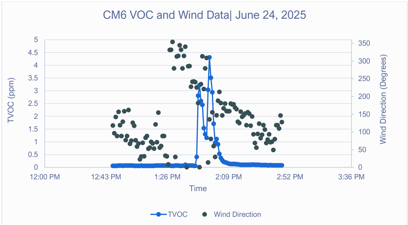
Figure 2 CM6 – Focus Points tVOC and Wind Direction June 24, 2025, 12:48 PM to 2:47 PM
