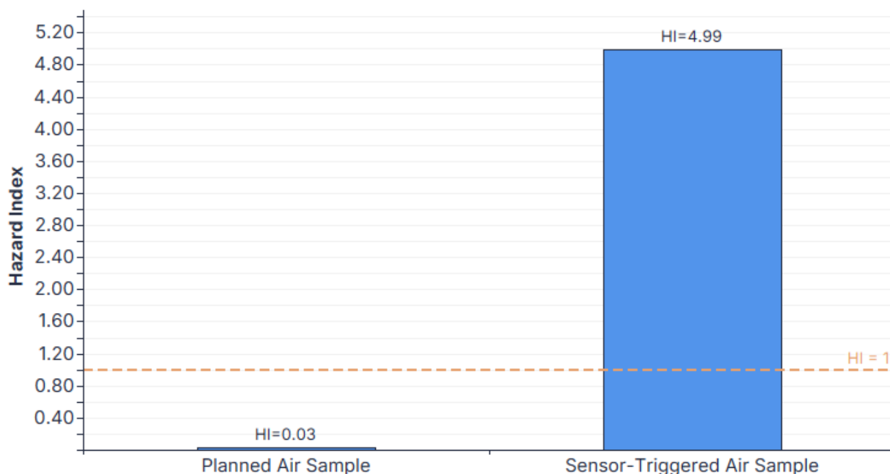
Figure 6 Hazard Indices at the CCND CM6 – Focus Points for Planned (June 3, 2025) and Sensor-Triggered (June 24, 2025) Air Samples
