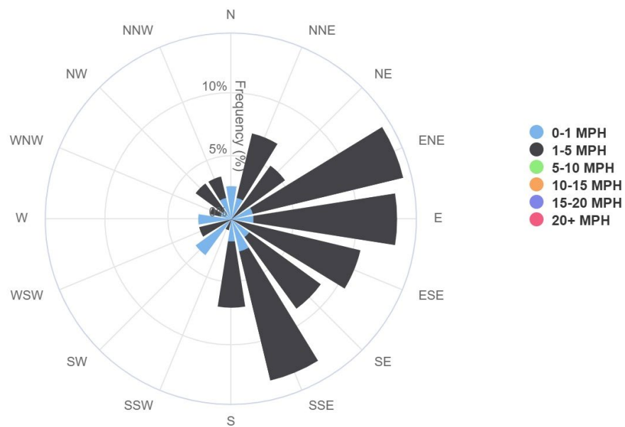
Figure 3 CM6 – Focus Points Wind Rose June 24, 2025, 12:48 PM to 2:47 PM
